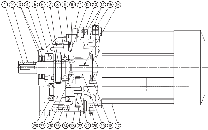
Fig F-21 Type CHHM (6000SK Series Horizontal, Gearmotor) (Example: Frame size 6075SK)
