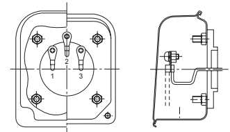
3-Phase indoor terminal box
