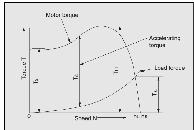
Fig F-9 Torque Curve
